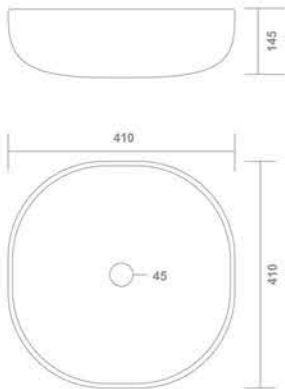
2017-ATLAS Table Top Basin 410x410x145mm
